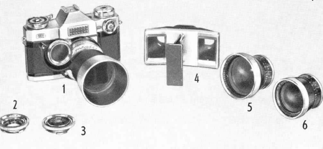
Fig. 28 1. CONTAFLEX super with close-up STERITAR-B (with Proxar f = 0.5 m in the swung-out filter trap) 2. Front element of TESSAR f/2.8 , 50 mm, which is part of the basic camera equipment. 3. PRO-TESSAR M 1 : 1 4. STERITAR-B with separator 5. PRO-TESSAR f/4 , 35 mm 6. PRO-TESSAR f/4 , 85 mm
